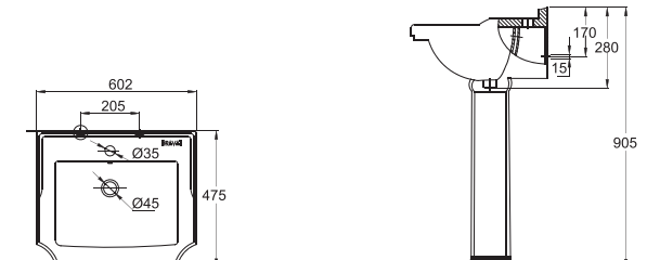
C22162W-1 60CM BASIN / PEDESTAL 602X475X905mm
