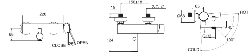
F63368C-01 WALL-MOUNTED BATH & SHOWER FAUCET BODY
