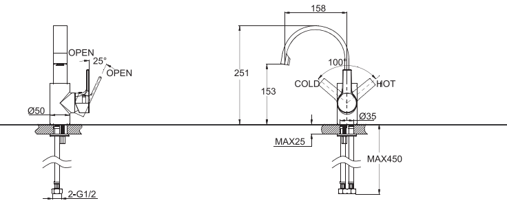
F13379C SINGLE LEVEL LAVATORY FAUCET
