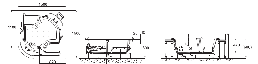
B25510W-4 1.5M BUILD IN MASSAGE BATHTUB 1500X1500X600mm
