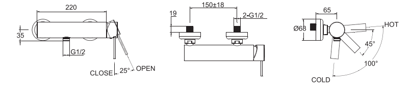
F93368C-01 WALL-MOUNTED SHOWER FAUCET BODY
