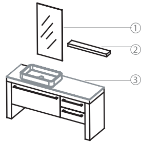
MA005-1 150CM SINGLE DRAWER DARK-GREY CABINET SET ① M225N 900X450X6mm ② M0430K 700X120X45mm ③ MA005 1500X450X730mm Recommand mixer F15051C +D915C /F16061K-A
