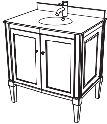
MA011 85CM CLASSIC CABINET W/STONE TABLE TOP 850X610X930mm Recommnd mixer F12680C /F11251C
