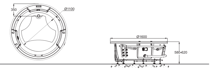
B25615W-4 1.6M BUILD IN MASSAGEBATHTUB 1600X1600X600mm
