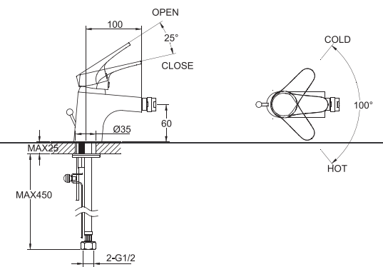
F32634C SINGLE LEVER BIDET FAUCET
