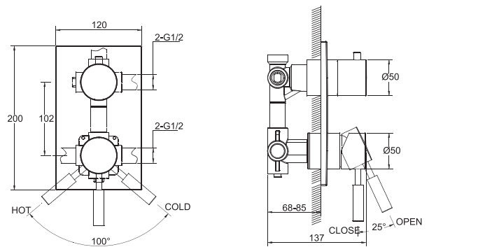
FB85151C-2 IN-WALL 2 WAY FAUCET BODY
