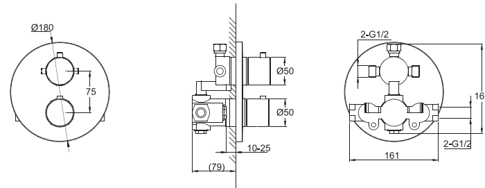
FB84062C THERMOSTAT WALL-MOUNTED FAUCET BODY
