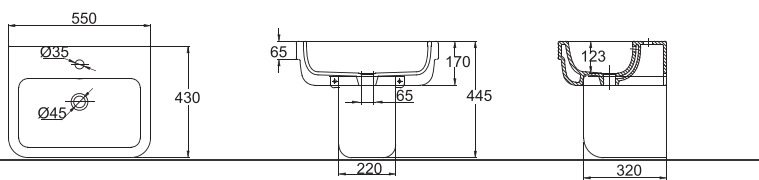
C22133W-1 55CM BASIN / SEMI- PEDESTAL 550X430X445mm
