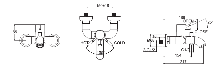
F61212C-01 WALL-MOUNTED SHOWER FAUCET
