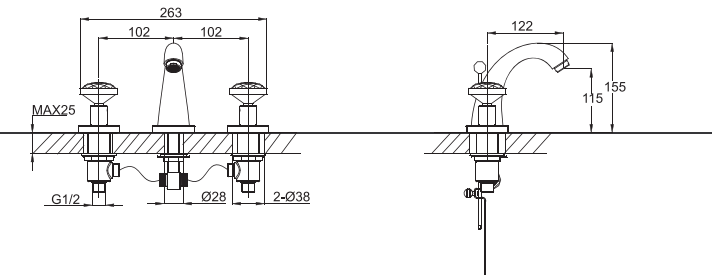
F21180C 3 PCS WIDESPREAD LAVATORY CRYSTAL FAUCET
