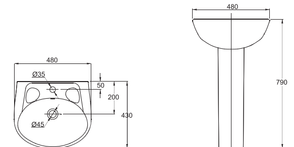
C22139W-1 48CM BASIN / PEDESTAL 480X430X790mm
