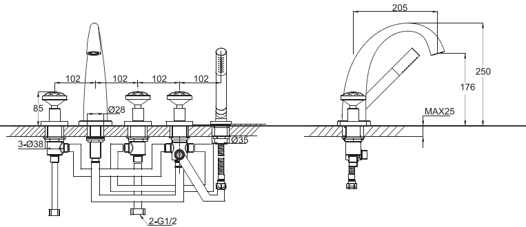
F51180C 5PCS BATH CRYSTAL FAUCET
