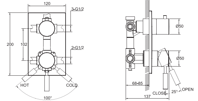
FB85151C-3 IN-WALL 3 WAY FAUCET BODY
