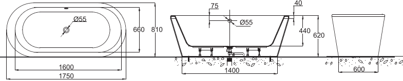
B25801W-1 1.75M FREE STANDING BATHTUB 1750X810X620mm
