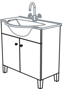
MA015 ENGRAVED CABINET 820X465X865mm Recommnd mixer F12680C /F11251C M231Y
