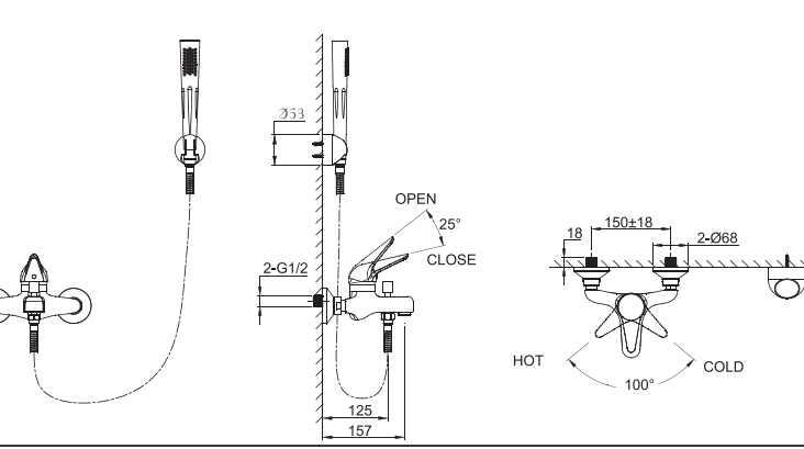
F62754C WALL-MOUNTED BATH & SHOWER FAUCET
