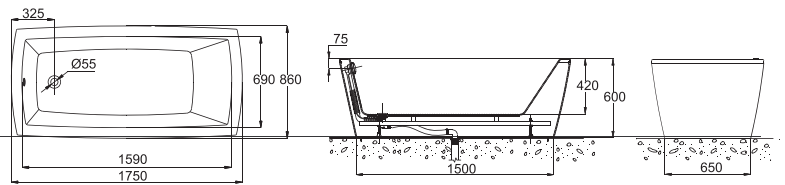
B25807W-1 1.75M FREE STANDING ACRYLIC BATHTUB 1750X860X600mm
