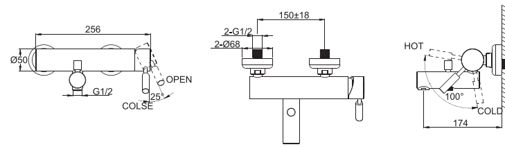
F61251C-01 WALL-MOUNTED BATH & SHOWER FAUCET BODY
